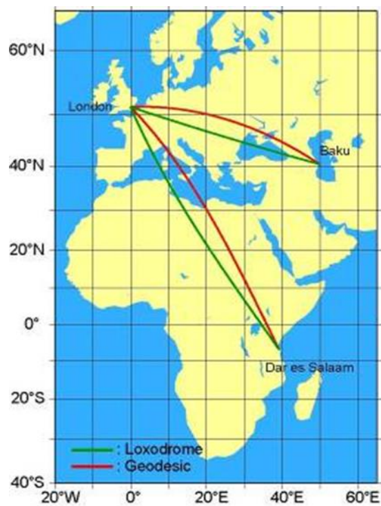
Figure 3. 5 - Loxodrome and geodesic on a Mercator chart
