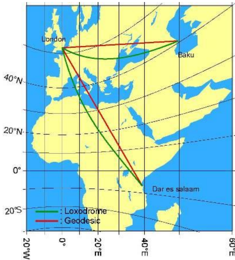
Figure 3. 7 - Loxodrome and geodesic on a gnomonic chart
